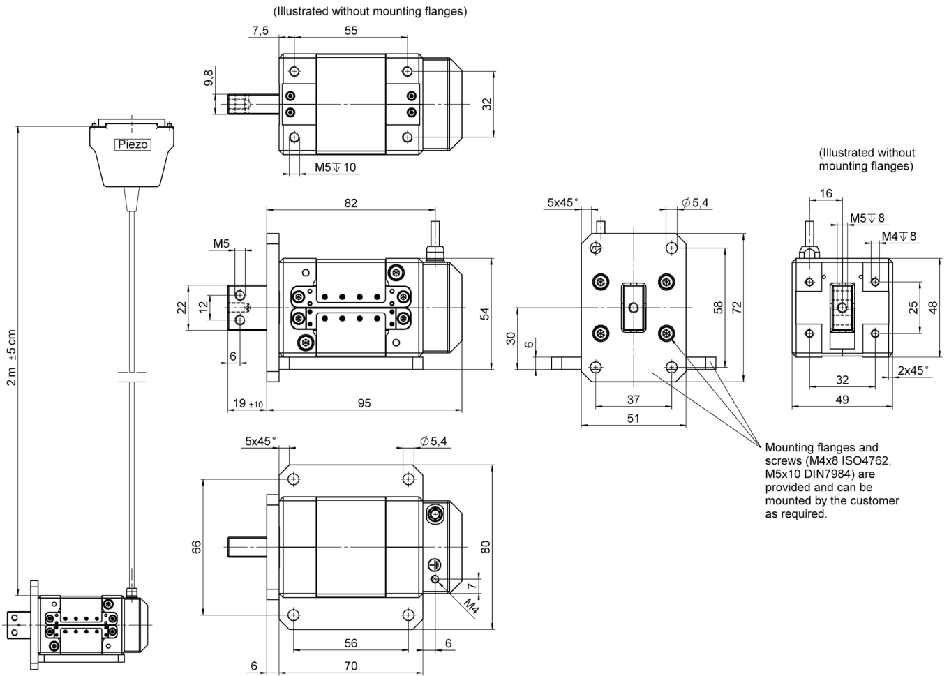
N-216, dimensions in mm. Mounting flanges for side or front mounting are included in the delivery.
