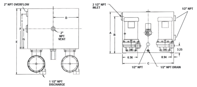
J series 30-120 gallon tanks
