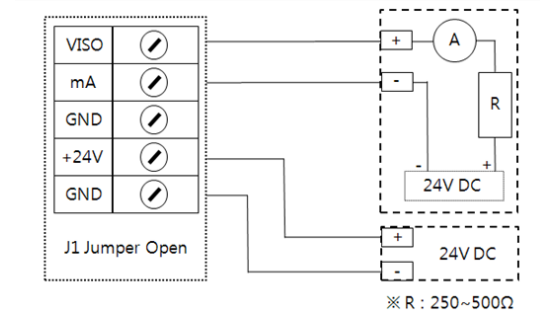
[Figure 5. 4~20mA Sink Driver Outline]
