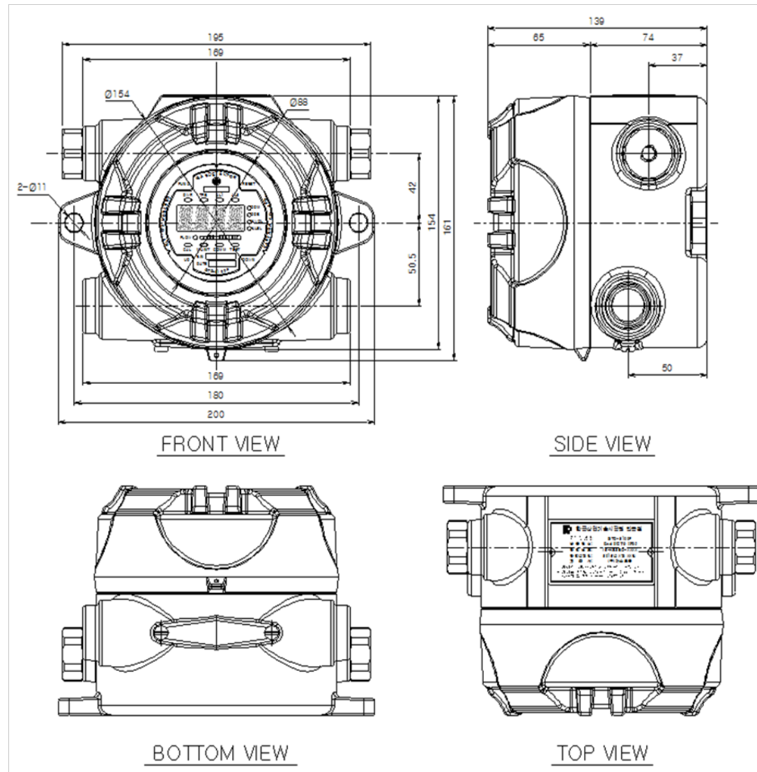
[Figure 7. GTD-5100F Drawing and Dimensions]
