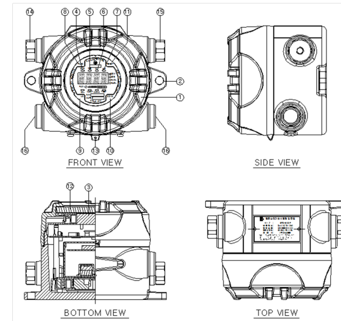
[Figure 2. GTD-5100F Components]
