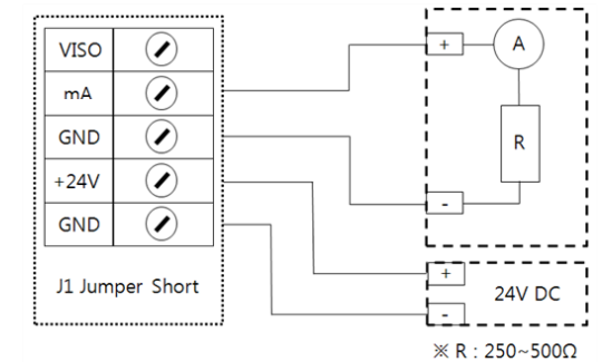
[Figure 4. 4-20mA Source Driver Configuration]
