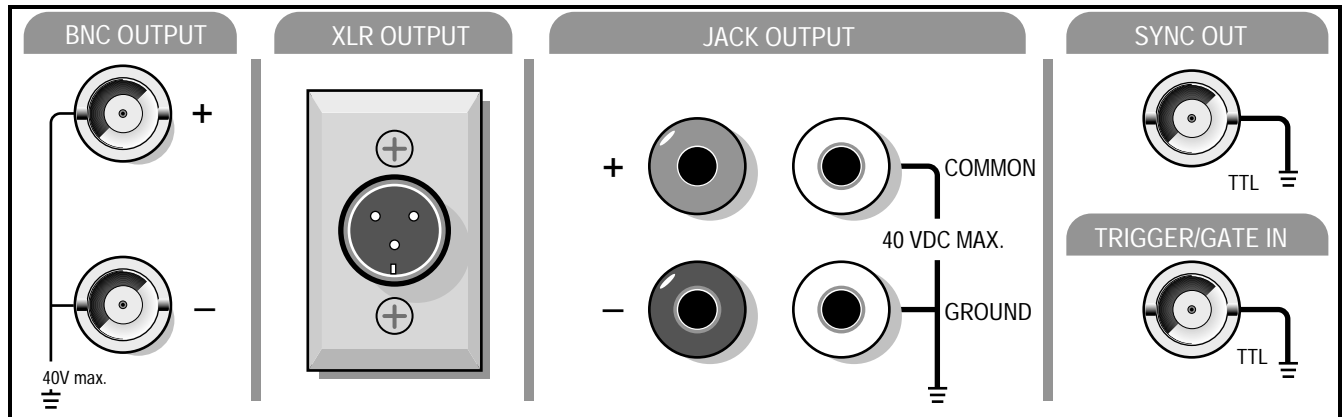
Figure 2-4 Outputs
