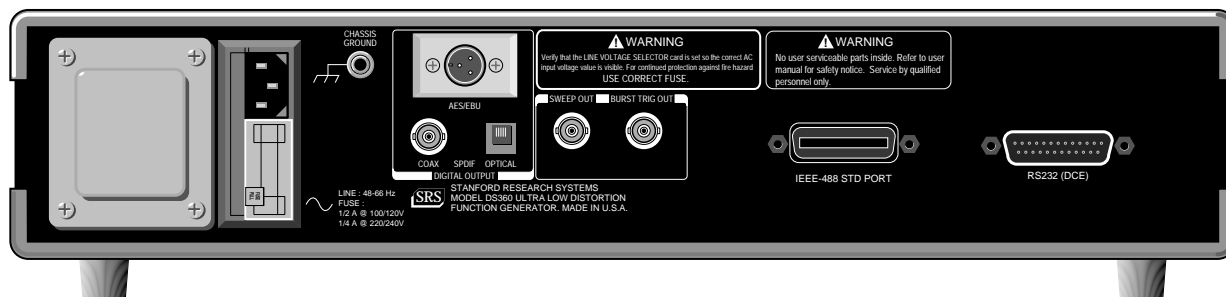
Figure 2-7 Rear Panel
