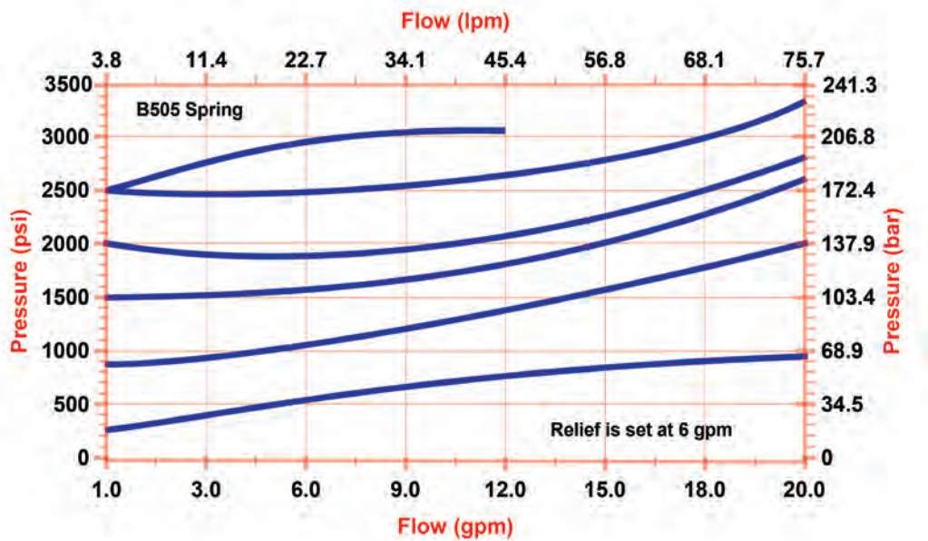
Pressure VS. Flow for AO Relief (R)
