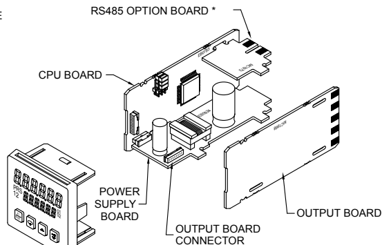
Figure 6, Relay Output Board Replacement
