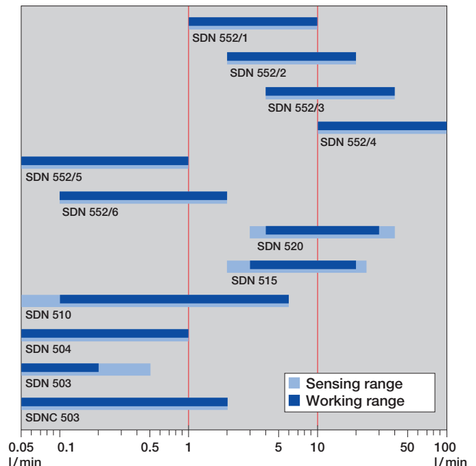
Flow ranges for EGE-Inline-Compact models
