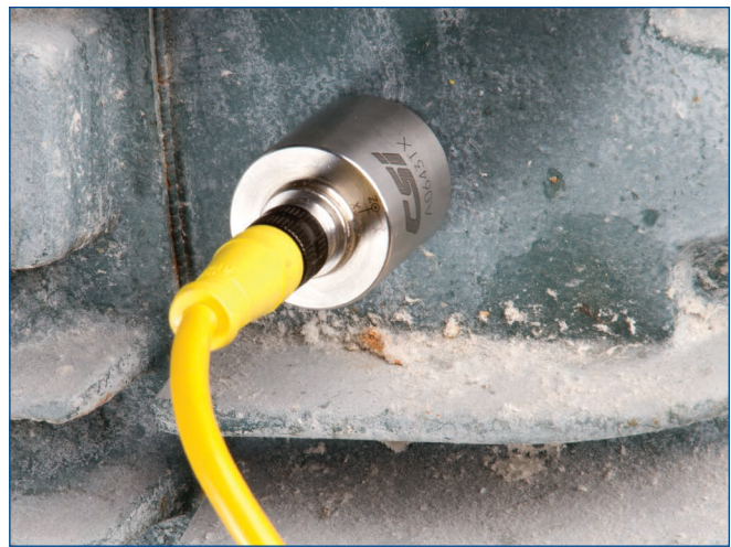
The triaxial accelerometer collects data at the measurement location from a vertical, horizontal, and axial directions simultaneously.
